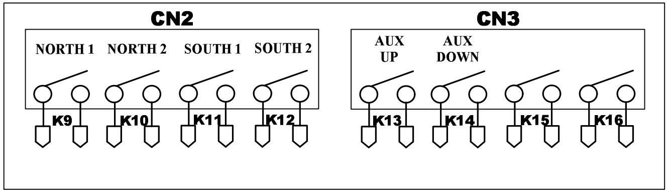
Relay Card 2
