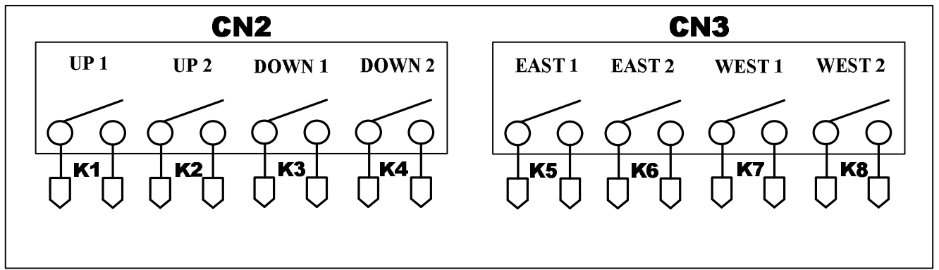
Relay Card 1
