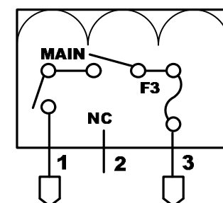
MAIN RELAY
